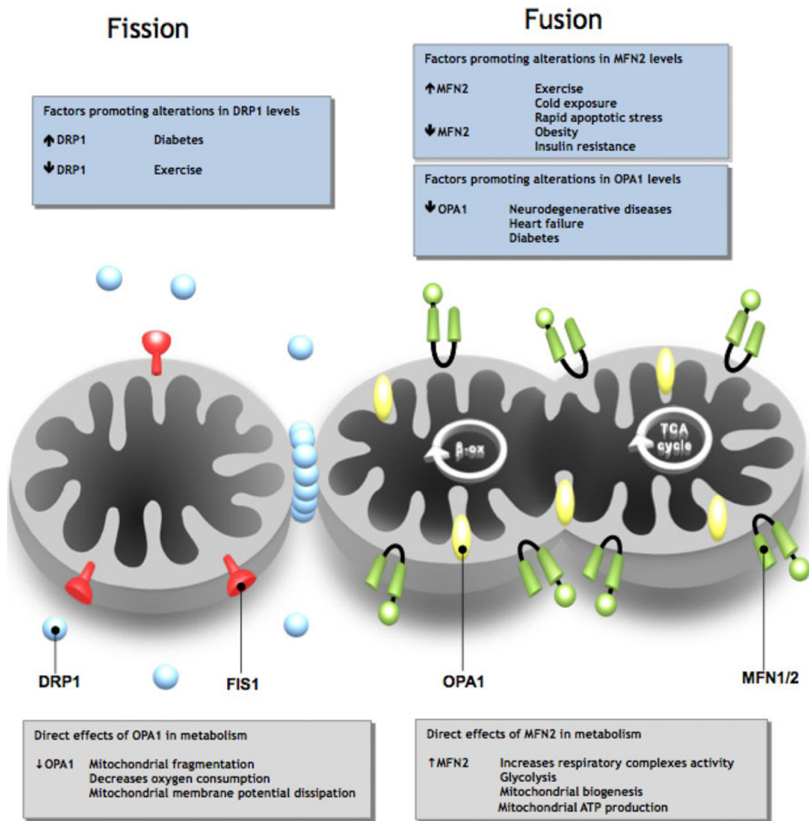
Fig. 1 Potential roles of mitochondrial dynamics in cardiac metabolism. Factors regulating mitochondrial fission and fusion are depicted at the left and right side of the figure, respectively. DRP1: Dynamin-
